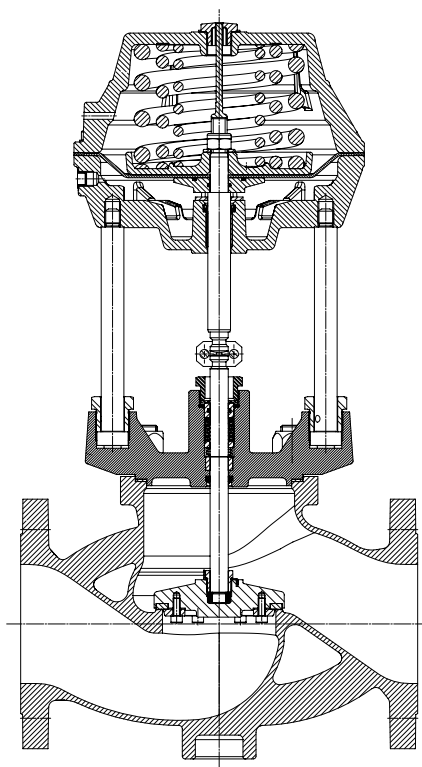
Sectional view
